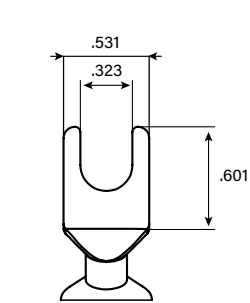
U-Spade Dimensions (in.)
