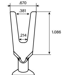
V-Spade Dimensions (in.)
